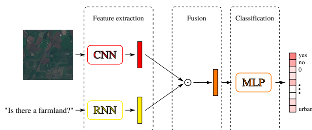
Fig. 2. Visual Question Answering model. In our experiments, the CNN is a ResNet-50 model [4] with a two layers fully-convolutional network to produce the feature vector, the RNN is a skip-thoughts model [5] and the fusion is a simple point-wise multiplication.
