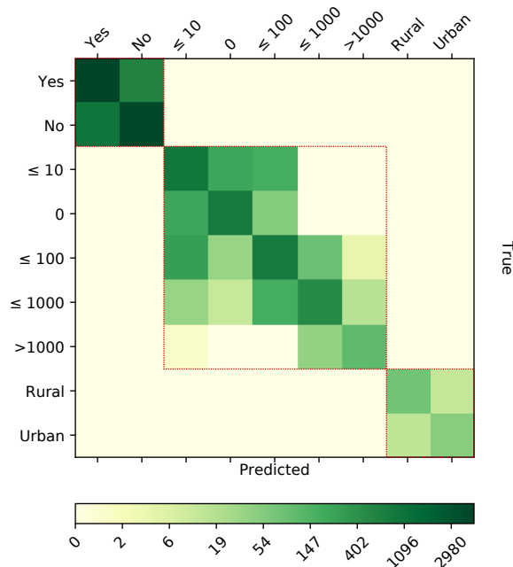
Fig. 3. Confusion matrix of the answers provided by the proposed model on the test set (logarithm scale). Dashed lines group answers by type ("Yes/No", numbers and "Rural/Urban").
